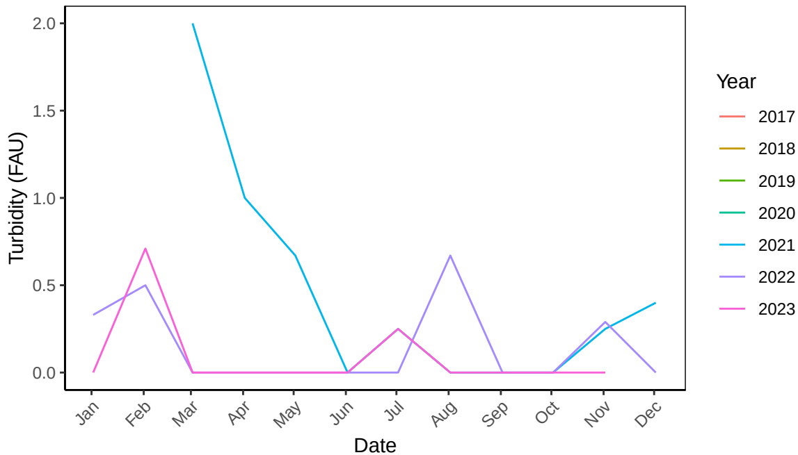
B2 Raceway 2 Turbidity (FAU) Monthly Statistics
